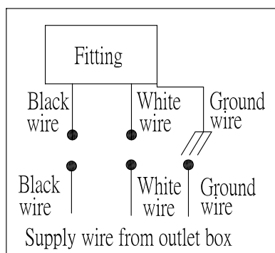
Circuit diagram 1
